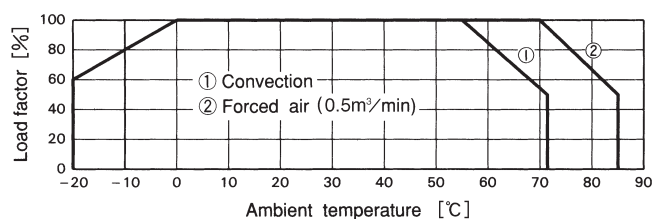
Fig.5.2 Derating curve
