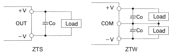
Fig.3.2 Connecting method of external capacitor at output terminal
