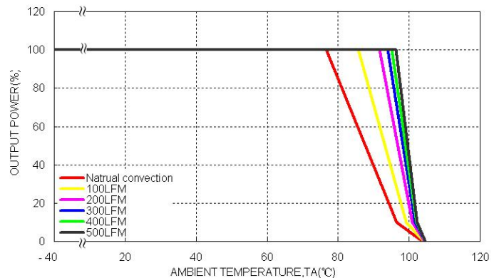
RED20-48S05W Derating Curve With Heat-sink ( Note 8 )
