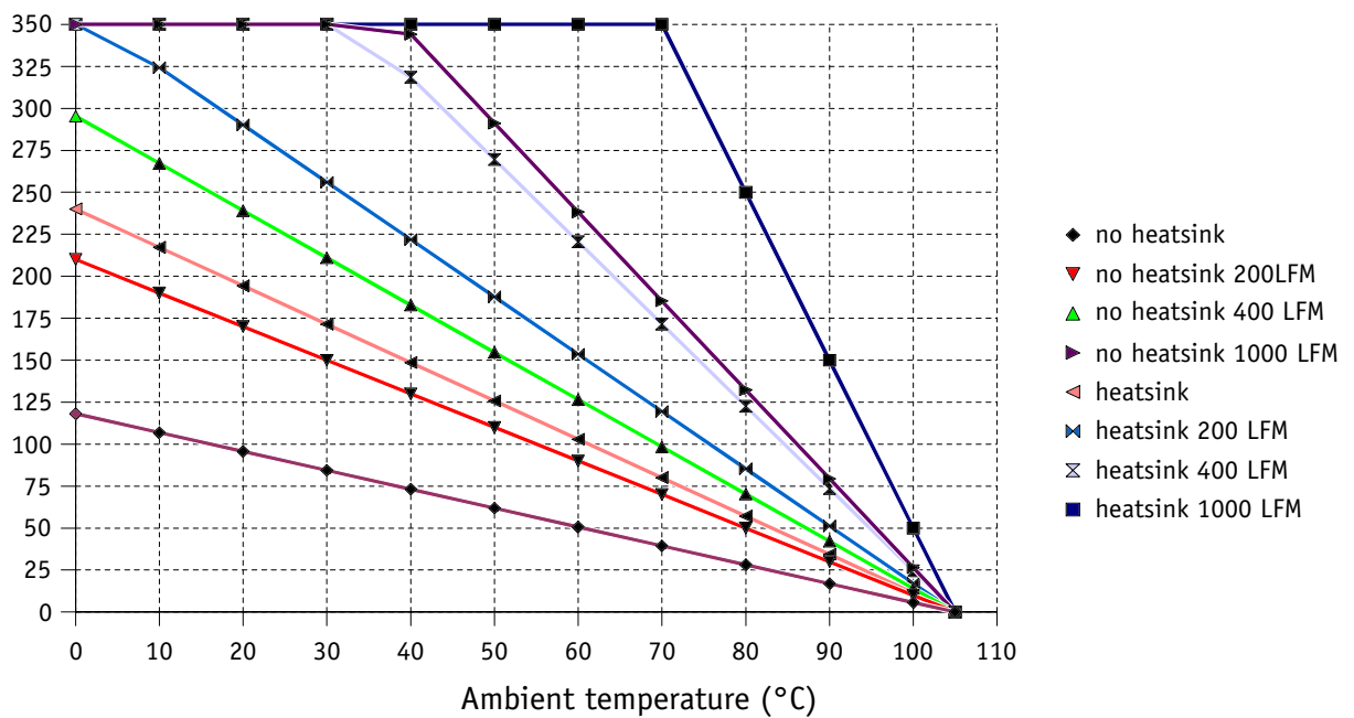
HGMS-350 Thermal Curves
